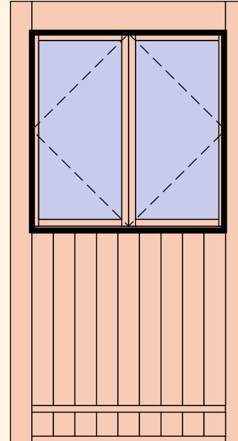
Glazed shutter to open from midrail. Fixed panels below
